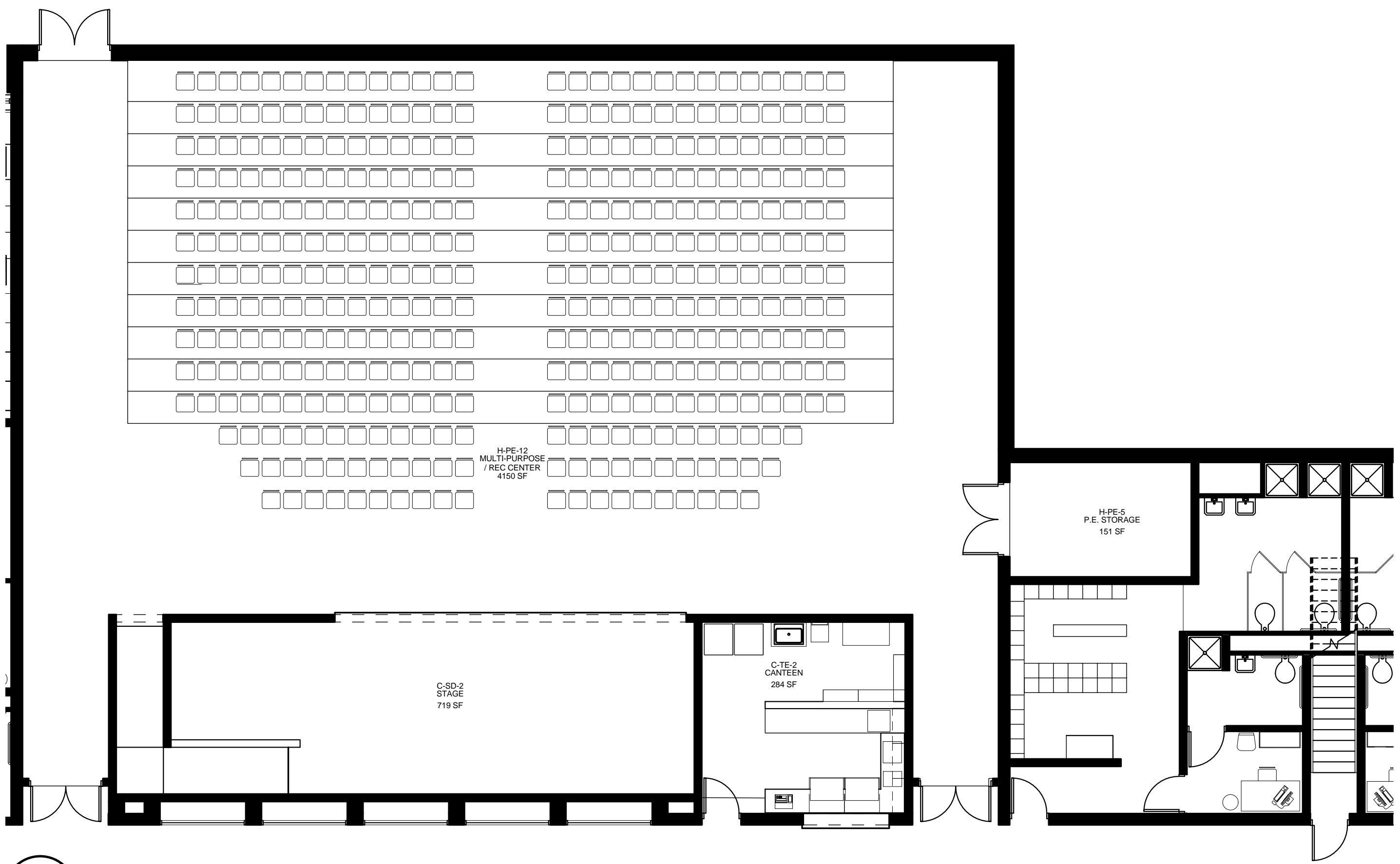
1 MULTI PURPOSE ROOM - SEATING LAYOUT - PARTIAL PLAN-OSD A-17.1 1/8" = 1'-0"
