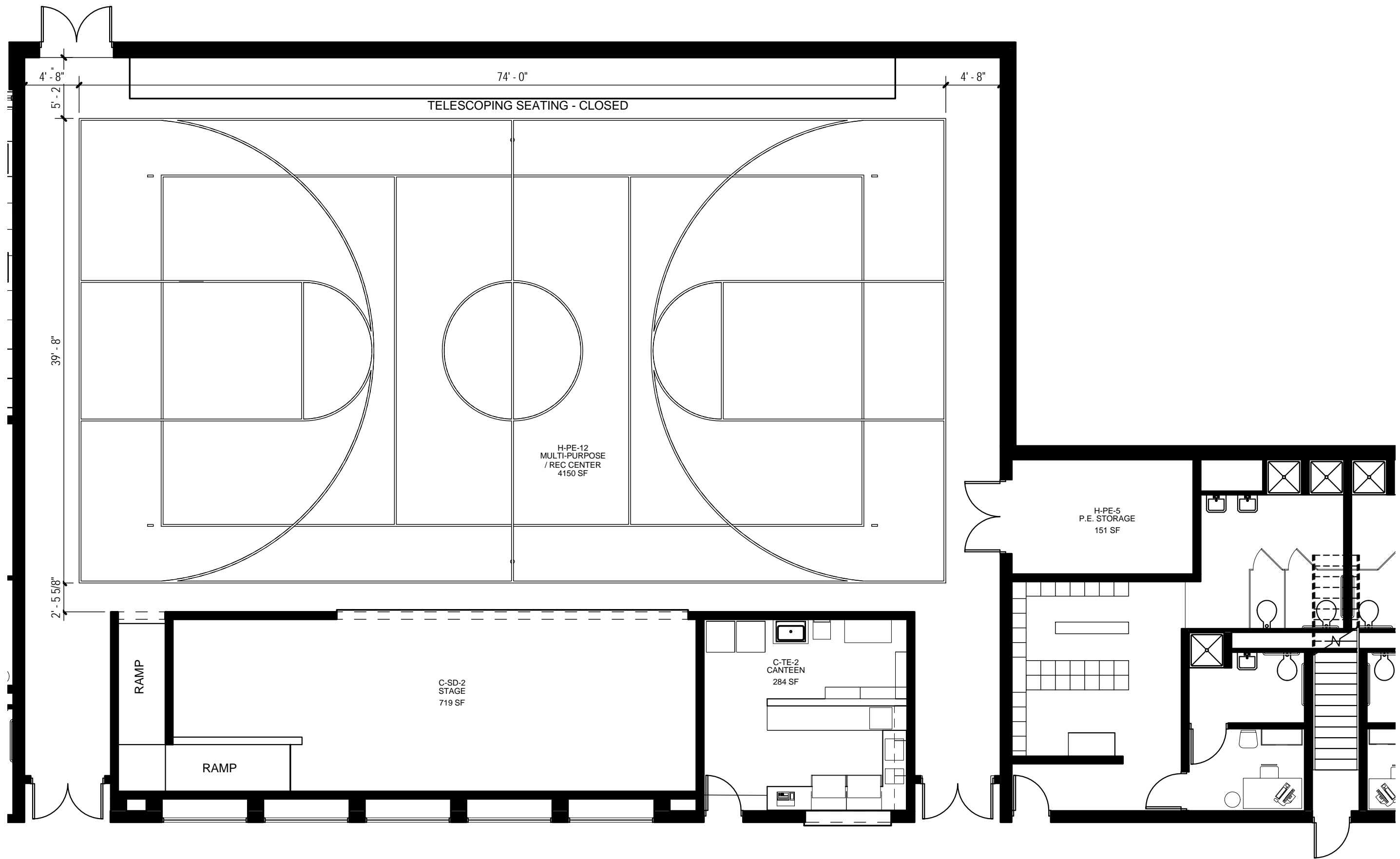
1 MULTI PURPOSE ROOM - COURT LAYOUT - PARTIAL PLAN-OSD A-17 1/8" = 1'-0"
